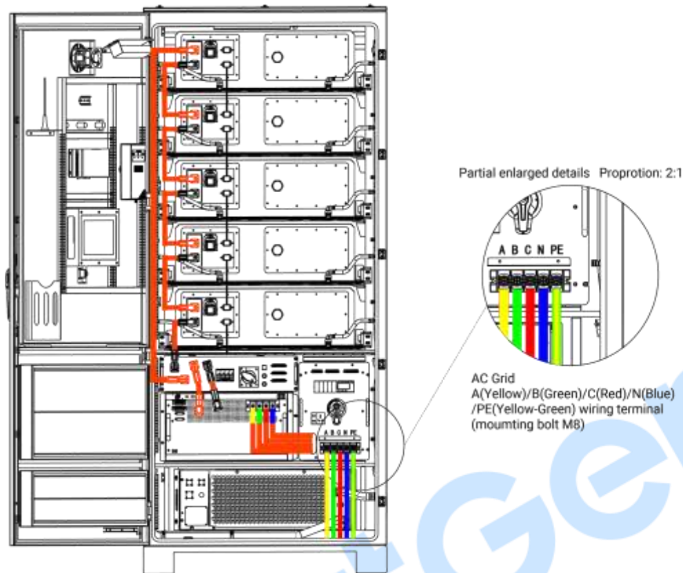
Fig.10 Wiring Terminal Diagram at AC Grid
