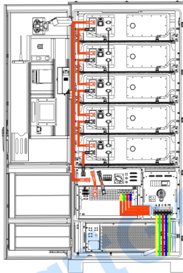
Fig.9 Power, Communication Line Connection Diagram Between Battery Box
