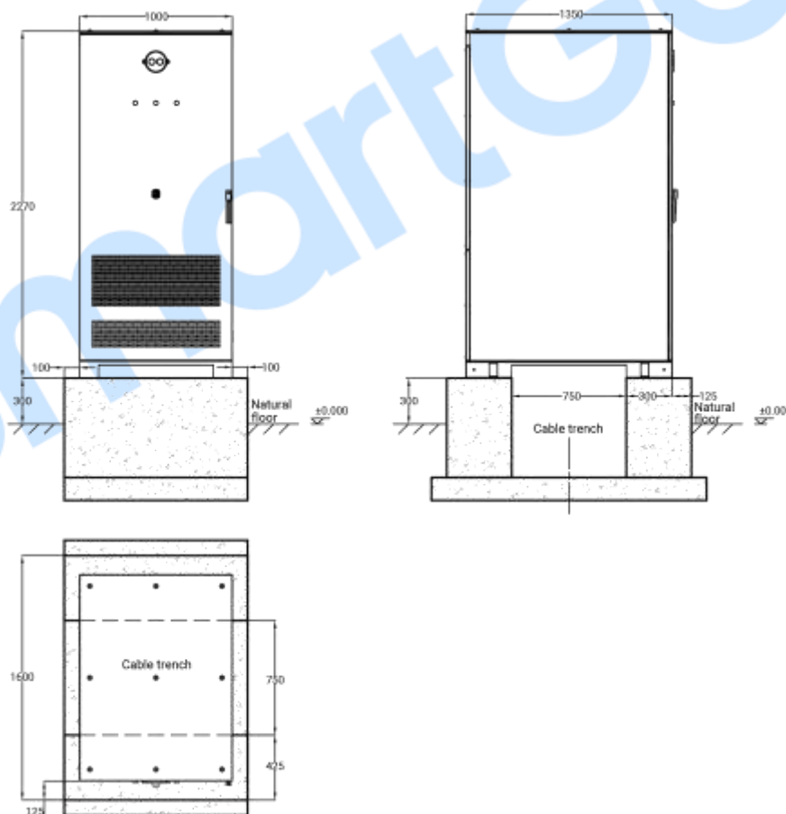
Fig.7 Reference Drawing of the Base Installation Size
