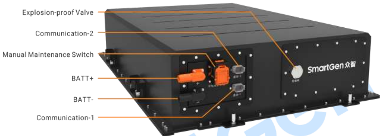
Fig.5 LCS Battery Box Appearance
