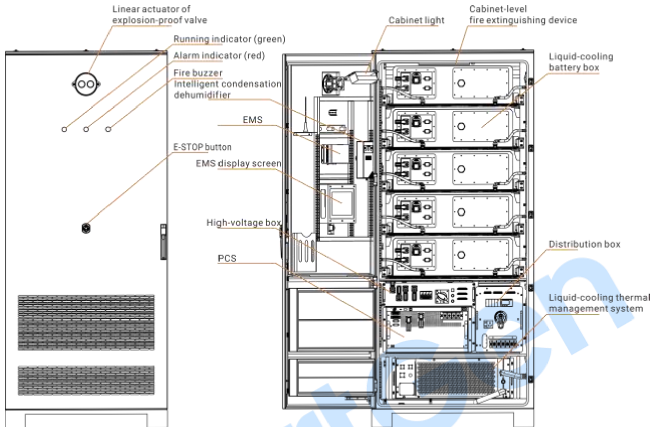
Fig.4 Main Equipment
