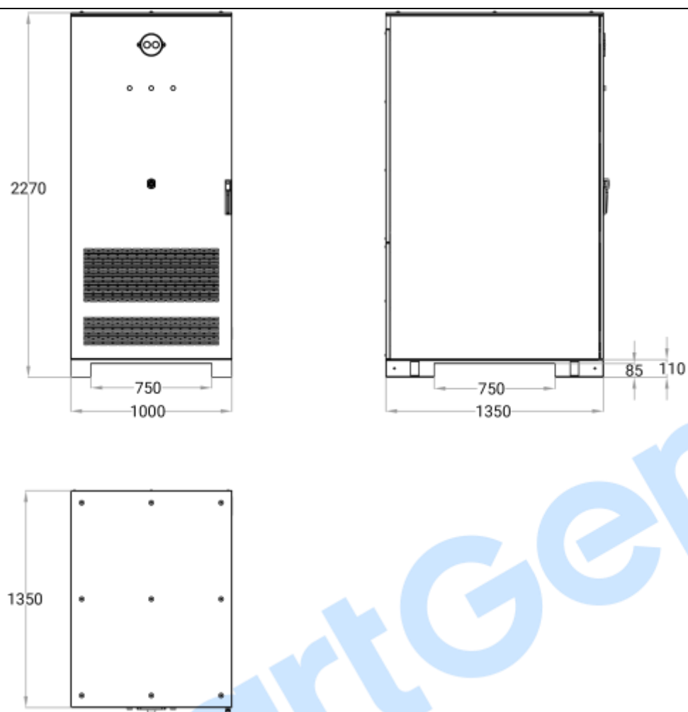
Fig.3 Overall Dimensions
