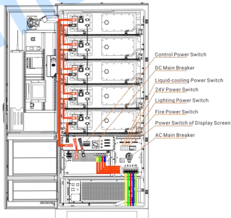
Fig.11 Operation Switch Position Diagram
